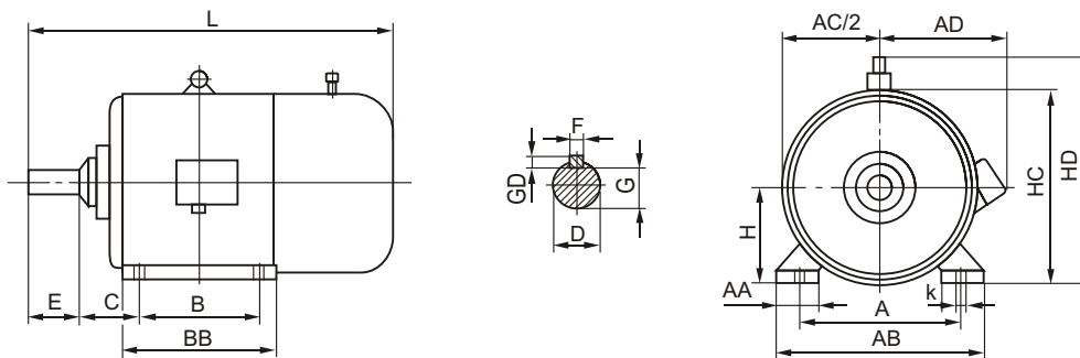
图1 YEJ系列 (B3) (见表3) Figure 1 YEJ Series (B3) (See table 3)
