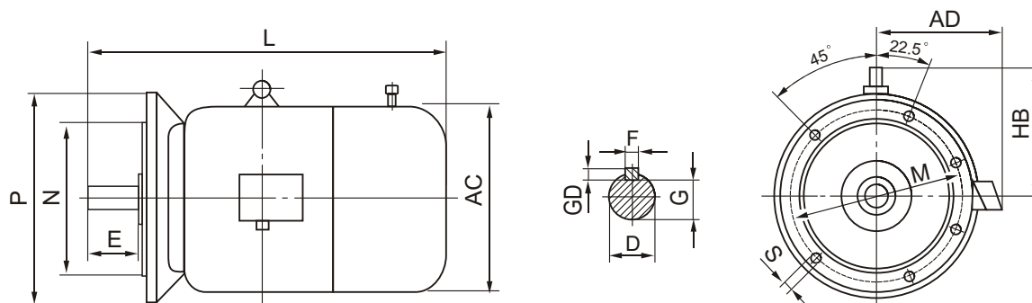
图2 YEJ系列 (B5) (见表4) Figure 2 YEJ Series (B5) (See table 4)
